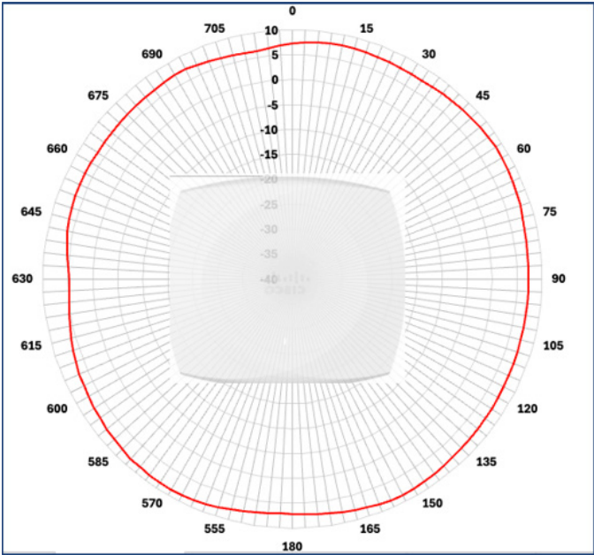
Figure 2. 5-GHz slot 2 radio antenna patterns
