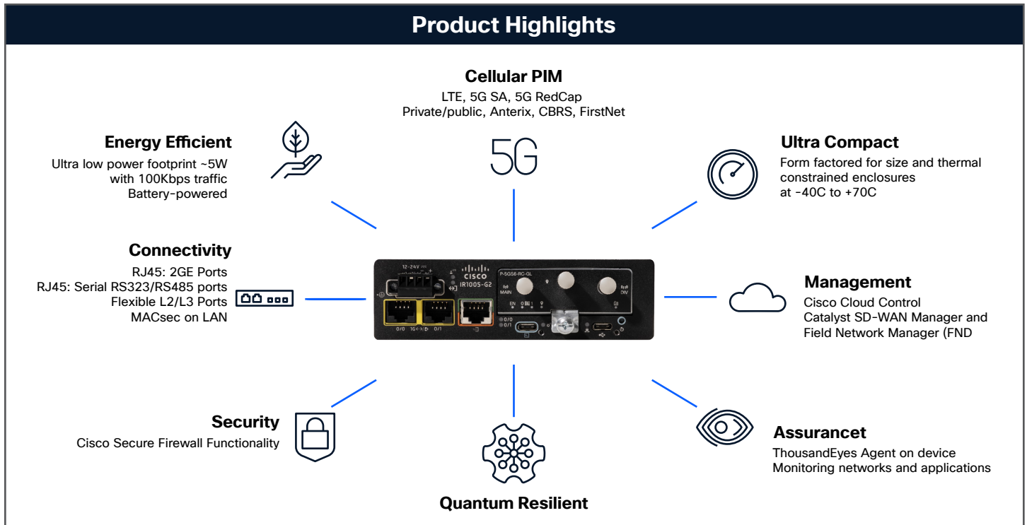
Figure 2. Cisco IR1000 product highlights
