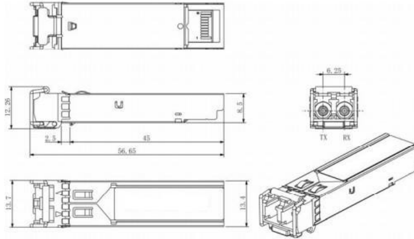
Mechanical Drawing
