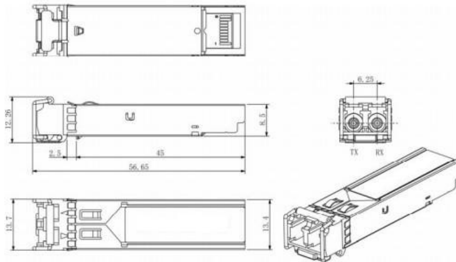
Mechanical Drawing
