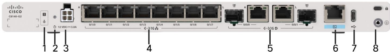
Figure 4. Front View of a Cisco C8140-G2 Secure Router
