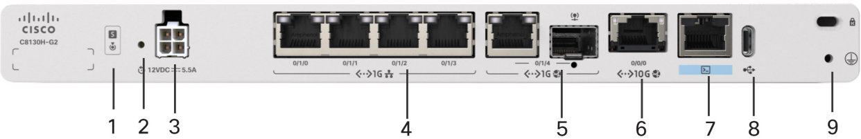
Figure 2. Front panel of Cisco C8130H-G2 Secure Router
