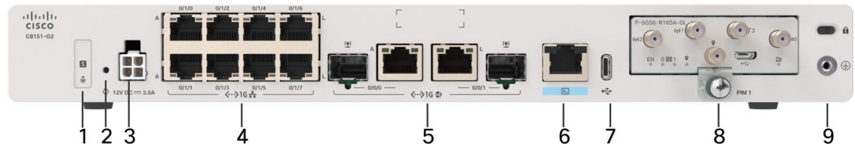
Figure 5. Front View of a Cisco C8151-G2 Secure Router
