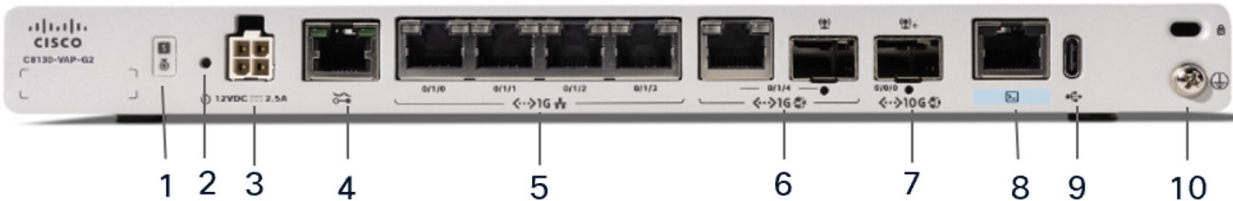
Figure 3. Front panel of Cisco C8130-VAI-G2/Cisco C8130-VAP-G2 Secure Router
