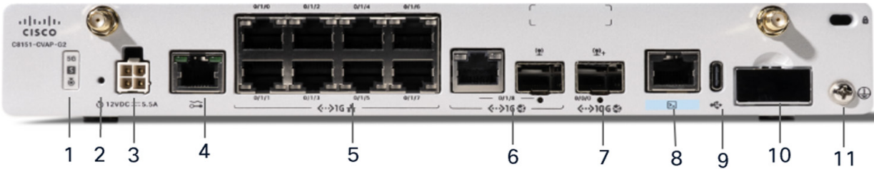
Figure 7. Front View of a Cisco C8151-CVAP-G2/Cisco C8151-CVAI-G2 Secure Router
