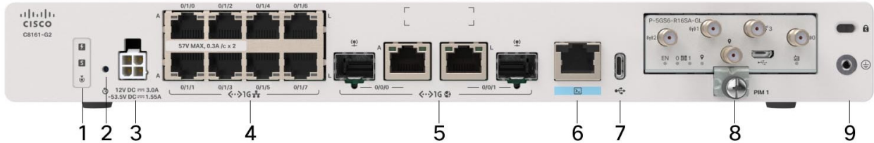
Figure 8. Front View of a Cisco C8161-G2 Secure Router
