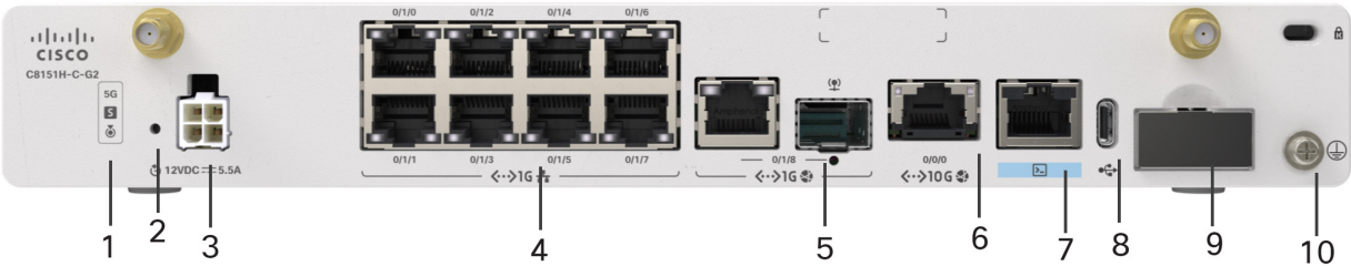
Figure 6. Front View of a Cisco C8151H-C-G2 Secure Router
